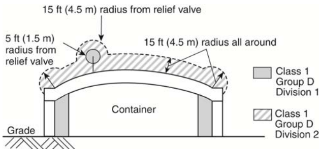
Figure A.10.7.2(d) Full Containment Container.
